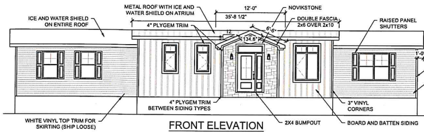
FRONT ELEVATION
